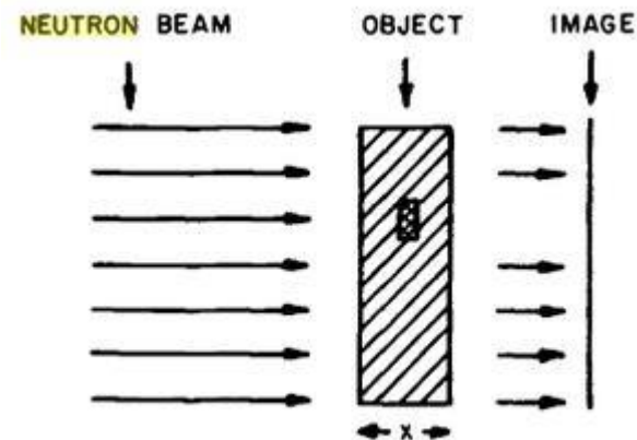
FIG. 1—The principle of neutron radiography.
