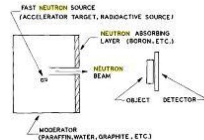
FIG. 1—Typical arrangement for thermal neutron radiography using an accelerator or radioactive neutron source. The detector is usually located directly behind the object.
